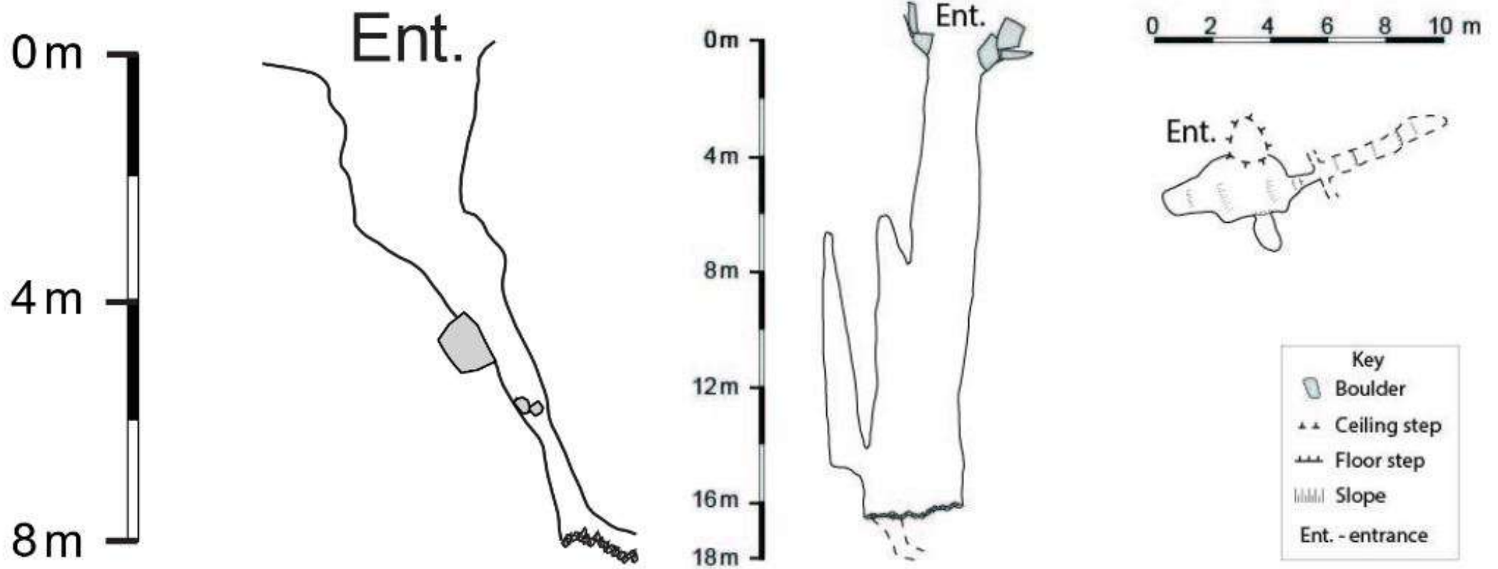
Figure 30. Sketch surveys of BA-1 (left) and BA-2 (right) that ended in chokes.
